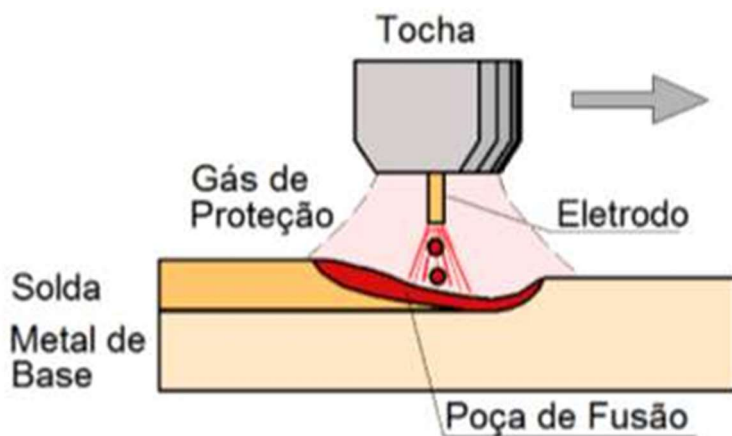
Figura 3 – Soldagem GMAW ( Gas Metal Arc Welding )
